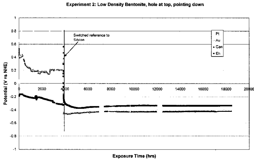
Example of electrochemical potential data obtained from one miniature canister with experiment.
