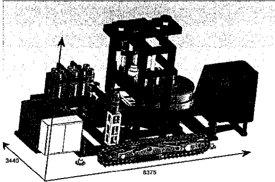
Artist impression of the drilling machine for deposition holes with preliminary dimensions.
