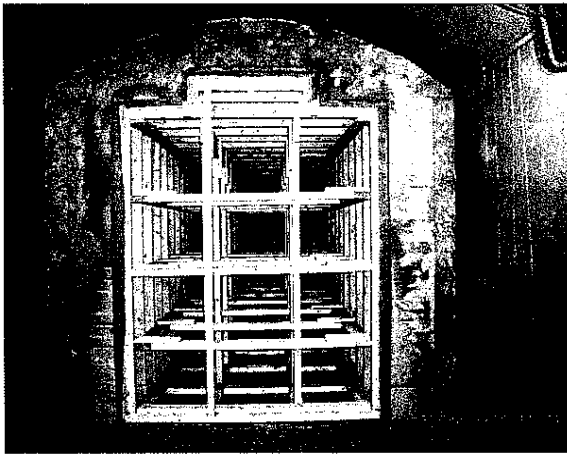
Test set-up for the deposition tunnel in half-scale.
