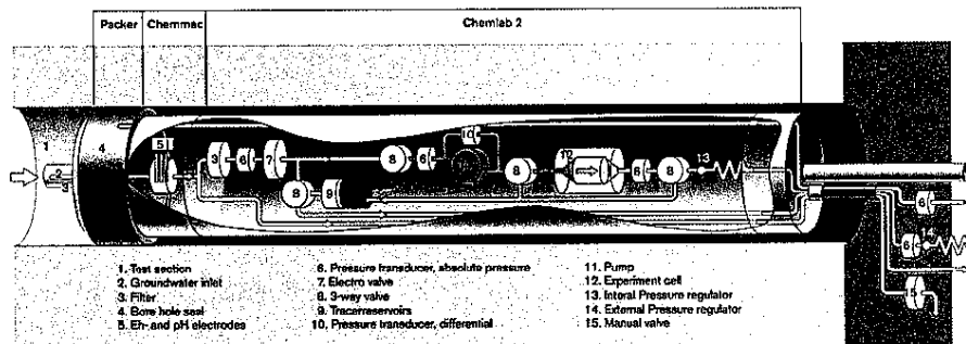
Principal drawing of Chemlab 2.
