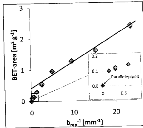
The specific surface area [ m^2 g^{-1} ] of chlorite as function of the inverse of the characteristic particle size [ mm^{-1} ]. The enlarged part of the plot shows results for larger particles.
