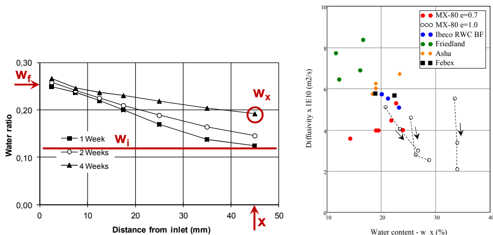
Figure 7-1. Water-uptake tests (left); evaluated diffusivity values (right).
