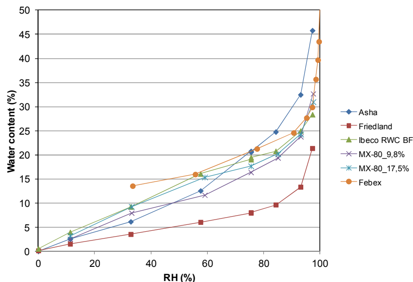
Figure 4-1. Retention data for different materials.
