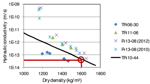
Figure 7-4. Evaluation of water-uptake tests with MX-80 bentonite ( w=11.5\% ; \rho_b=1590\text{ kg/m}^3 ; \rho_s=2780\text{ kg/m}^3 ).
