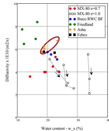
Figure 7-5. Evaluation of water-uptake tests with Asha bentonite ( w=17\% ; \rho_b=1600\text{ kg/m}^3 ; \rho_s=2900\text{ kg/m}^3 ).
