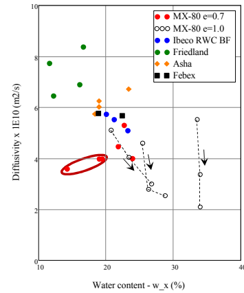
Figure 7-4. Evaluation of water-uptake tests with MX-80 bentonite ( w=11.5\% ; \rho_b=1590\text{ kg/m}^3 ; \rho_s=2780\text{ kg/m}^3 ).
