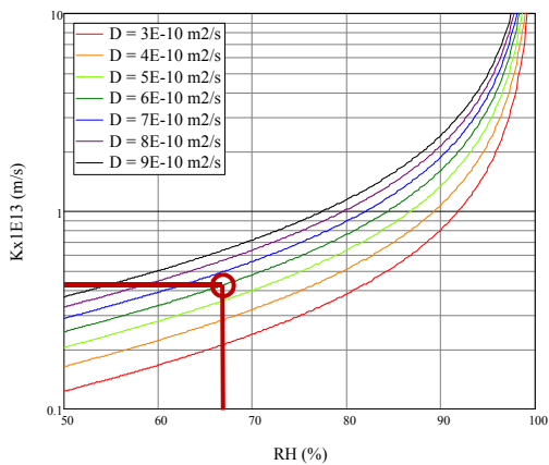
Figure 7-5. Evaluation of water-uptake tests with Asha bentonite ( w=17\% ; \rho_b=1600\text{ kg/m}^3 ; \rho_s=2900\text{ kg/m}^3 ).
