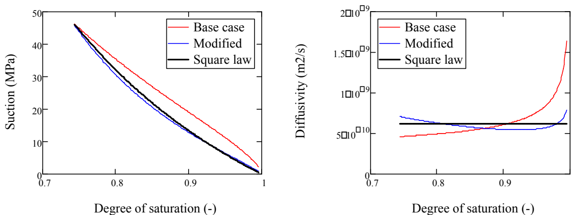
Figure 7-2. Retention curves, adopted for backfill blocks of MX-80 (left), and evaluated diffusivity relations (right).
