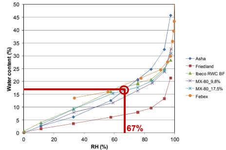
Figure 7-4. Evaluation of water-uptake tests with MX-80 bentonite ( w=11.5\% ; \rho_b=1590\text{ kg/m}^3 ; \rho_s=2780\text{ kg/m}^3 ).
