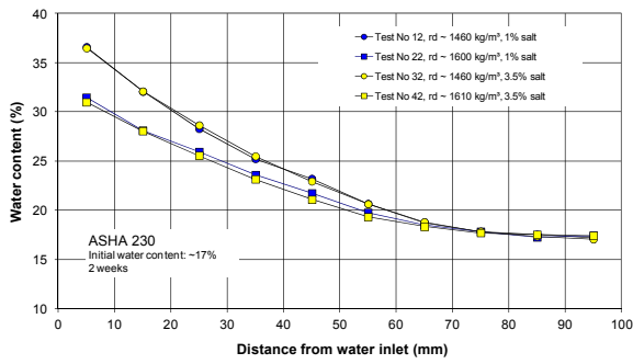
Figure 5-2. Water-uptake tests: Asha (left); Friedland (right).
