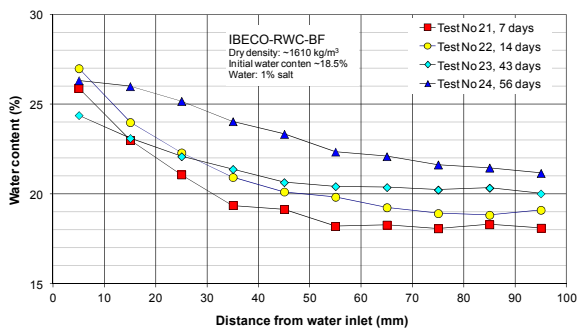
Figure 5-3. Water-uptake tests: Ibeco RWC BF.
