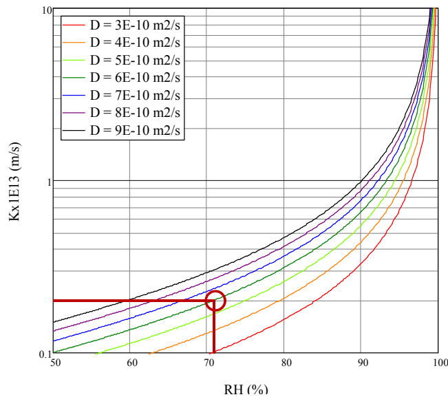
Figure 7-3. Hydraulic conductivity vs. initial RH for different D values. Data corresponding to backfill blocks with MX-80 ( w=17\% ; \rho_b=1700 \text{ kg/m}^3 ; \rho_s=2780 \text{ kg/m}^3 ).
