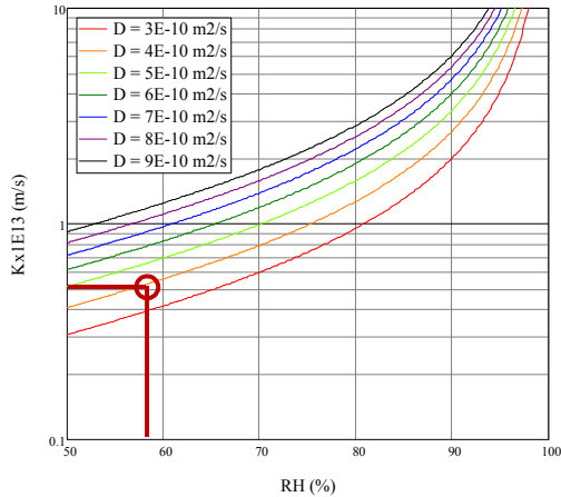
Figure 7-4. Evaluation of water-uptake tests with MX-80 bentonite ( w=11.5\% ; \rho_b=1590\text{ kg/m}^3 ; \rho_s=2780\text{ kg/m}^3 ).
