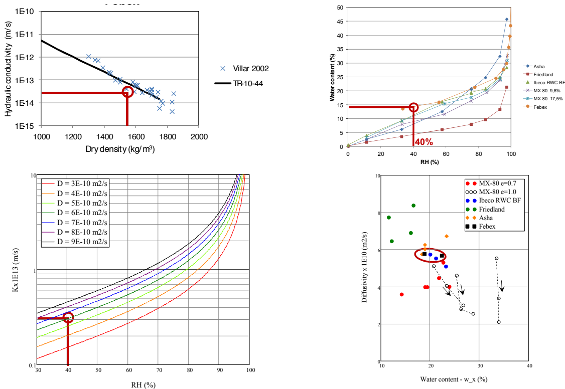
Figure 7-8. Evaluation of water-uptake tests with Febex bentonite ( w=14.3\% ; \rho_d=1551 \text{ kg/m}^3 ; \rho_s=2753 \text{ kg/m}^3 ).
