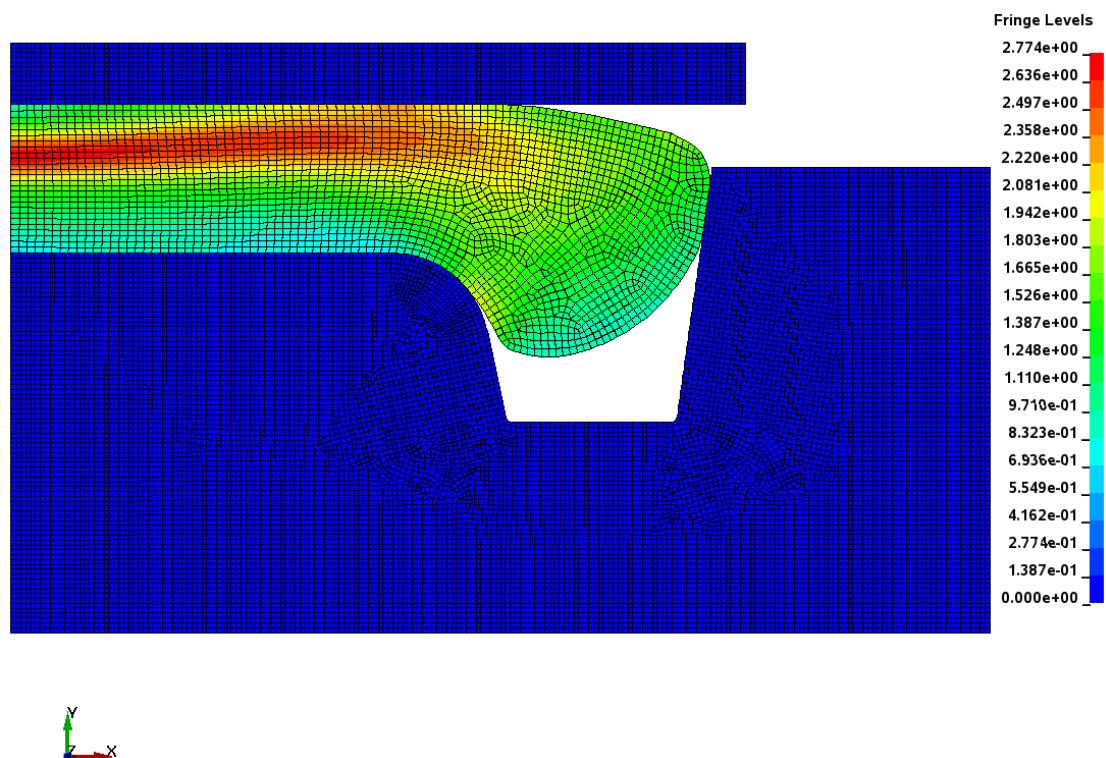
Figure 3-9. Effective plastic strain distribution for the reference method - step 4, closed die forging, at the final state where a maximum press force of 4,600 ton is reached.
