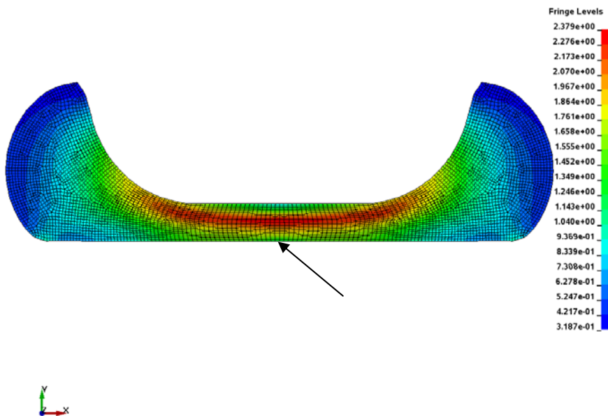
Figure 3-7. Effective plastic strain distribution for the case where plastic strains are not inherited from the previous step. An intrusion depth of 389 mm is applied during step 3 (minimum 70 mm remains). The arrow illustrates the lower center element referred to in the text. The model is mirrored in the yz-plane.
