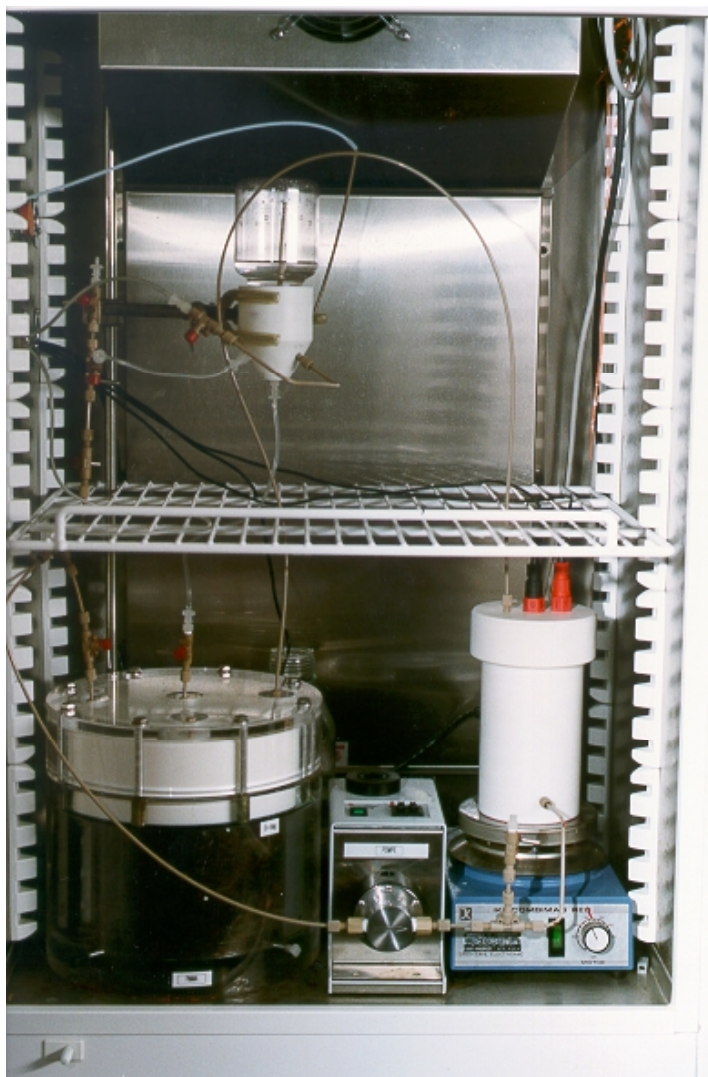
Figure 12. General view of the REPLICA set-up.
